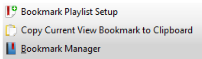
Bookmarking menu
